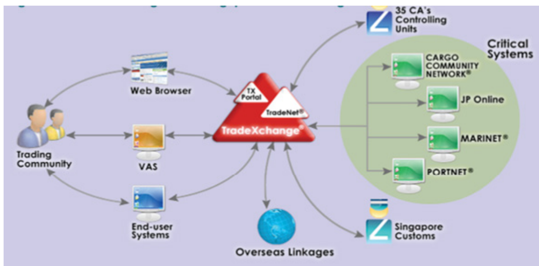
Figure 48: TradeXchange System
