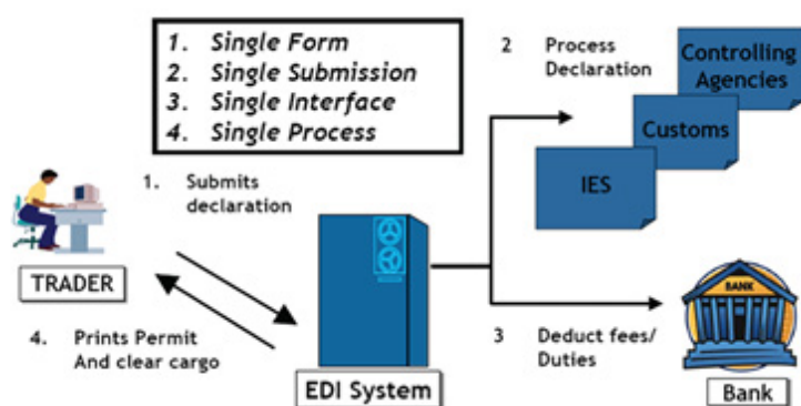
Figure 46: TradeNet System
